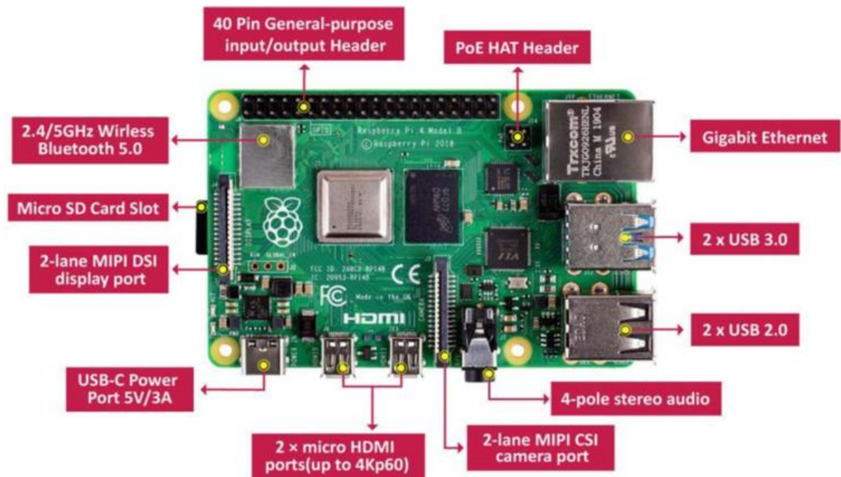
Labelling of Raspberry Pi:
